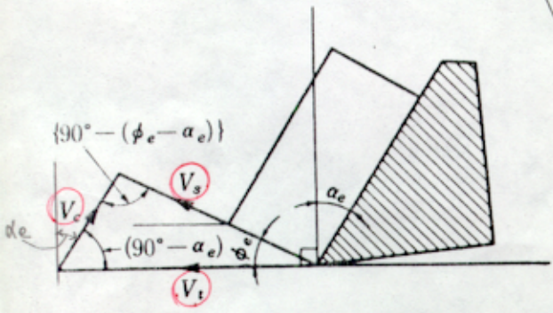
(b) true view of velocity plane
