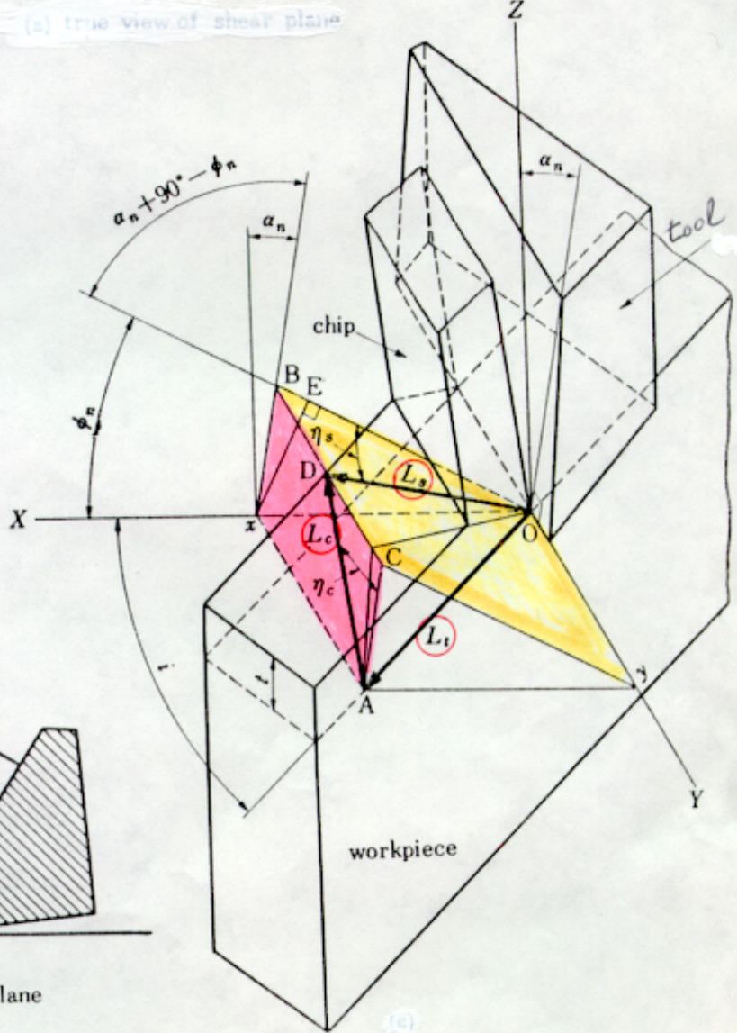
Fig. 2-11 chip formation in oblique cutting
